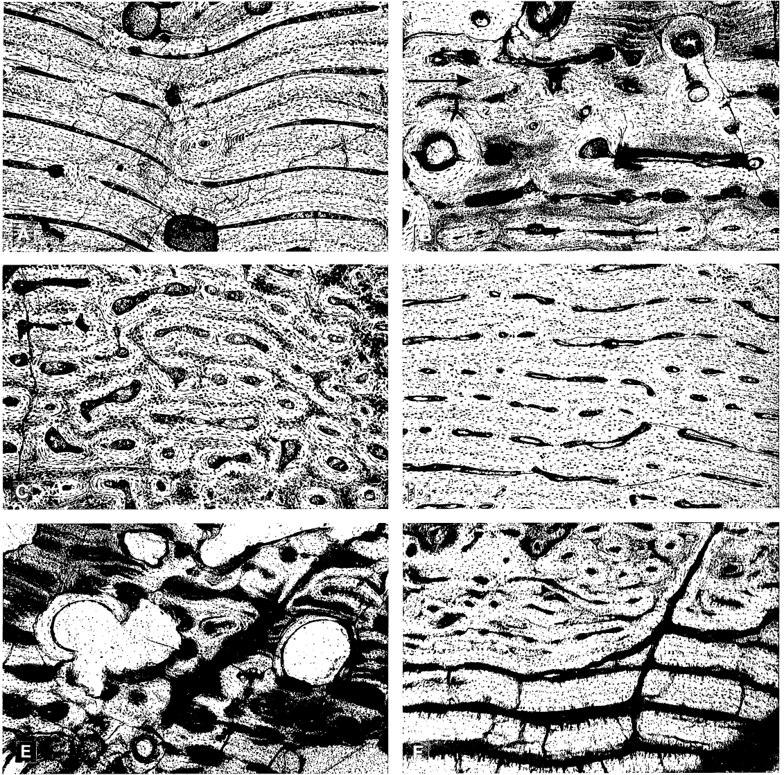
FIGURE 4. Differences in bone histology among the four saurpoid dinosaur genera from the Tendaguru beds (Upper Jurassic, Tanzania). The photomicrographs show the histology of various longbones at the middle of the diaphysis. The top of the frame is toward the bone surface. The width of all frames is 1.9 mm. A, Barosaurus humerus Ba4, type A, laminar fibrolamellar bone with narrow lumina of the outer cortex. B, Barosaurus femur Ba10, type B, laminar fibrolamellar bone with narrow lumina of the outer cortex with some secondary osteons and a line of arrested growth (arrows). C, Brachiosaurus humerus Br1, fibrolamellar bone with wide lumina of the middle cortex. D, Brachiosaurus humerus Br4, laminar fibrolamellar bone with narrow lumina of the outer cortex. E, Dicraeosaurus femur Di4, midcortex. Note the large cavities eroded into the fibrolamellar bone. They have only an incomplete lining of secondary bone. F, Dicraeosaurus femur Di4, fibrolamellar bone of the outer cortex with regions of differing vascular canal architecture.
