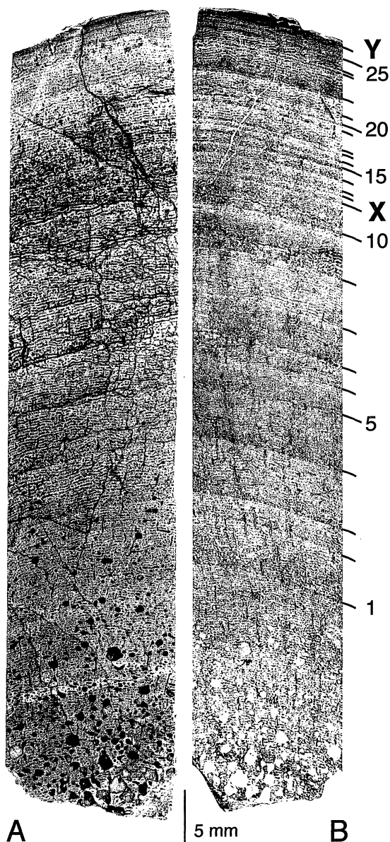
FIGURE 1. Photograph of polished section of Janenschia core femur Ja2. The bone surface is at the top. For ease of comparison, left image is reversed. A, Normal illumination. The laminar organization of the bone tissue is clearly visible. The erosional cavities in the inner cortex (bottom) are filled with clear calcite and appear dark. B, Reflection on the polished surface. Numerous polish lines (tick marks) are visible. The erosional cavities in the inner cortex (bottom) appear light because they create a large, even reflection. The count of the polish lines is based on examination of the core under a compound microscope using bright-field illumination. Note the wide spacing of the first 11 lines. X = presumable onset of sexual maturity as indicated by sudden decrease in polish line spacing. Y = change from fibrolamellar bone to lamellar-zonal bone, recording the near cessation of growth.
