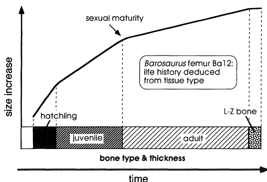
FIGURE 8. Change of bone type during ontogeny in a single Barosaurus (type A) femur, specimen Ba12. This bone is exceptional in that nearly the entire life history of the individual is recorded in a single location of the cortex. The changes in tissue type record the stepwise decrease in growth rate. The second decrease is best interpreted as the onset of sexual maturity. Size increase can only be plotted qualitatively because the exact relationship between cortex thickness at any one time and bone size is unknown.
